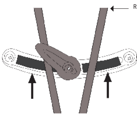
Mounting in semi ellipse of Quick-Lock1 system
