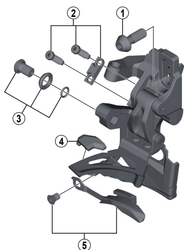
Low clamp
