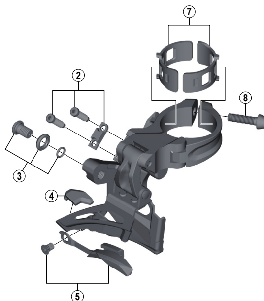
High clamp
