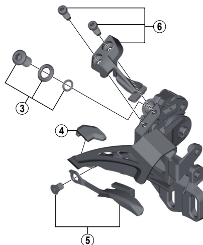
High clamp
